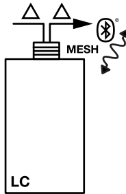
C-L20-00-00-17-DJ00 LOAD CONTROLLER ON/OFF 20A 2.2"x1.7"x1.1" (54x44x28mm) LINE INPUT 100-277VAC | OUTPUT 100-277VAC INSTALL WITHIN 30' OF CLOSEST DEVICE
