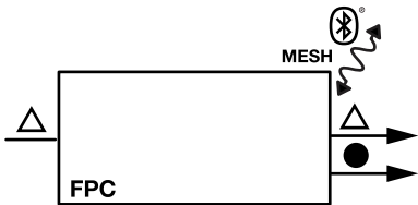
C-F00-11-DL00 FORWARD PHASE DIMMING CONTROLLER 5.25"x1.5"x1.25" (134x38x29mm) LINE INPUT 110-277VAC 200W MAX | AUXILIARY +24VC OUTPUT 100mA INSTALL WITHIN 30' OF CLOSEST DEVICE
