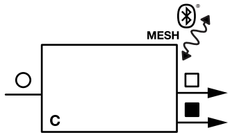
C-T1C-24-DS00 SINGLE CH 0-10V CONTROLLER 3.25"x1.5"x.25" (83x38x6.4mm) INPUT 12-24VDC | OUTPUT 0-10VDC 0-10V DIMMING 100mA MAX INSTALL WITHIN 30' OF CLOSEST DEVICE
