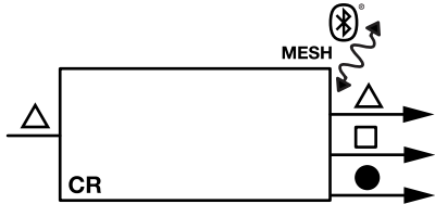
C-T1C-11-DL00 SINGLE CH 0-10V CONTROLLER WITH RELAY 5.25"x1.5"x1.125" (134x38x29mm) AC INPUT 110-277VAC OUTPUT RELAY 110-277VAC | 10 AMPS MAX 0-10V DIMMING 100mA MAX INSTALL WITHIN 30' OF CLOSEST DEVICE
