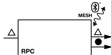
C-R00-11-DL00 REVERSE PHASE CONTROLLER 5.25"x1.5"x1.25" (134x38x29mm) LINE INPUT 110-277VAC 200W MAX | AUXILIARY +24VC OUTPUT 100mA INSTALL WITHIN 30' OF CLOSEST DEVICE
